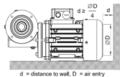
d = distance to wall, D = air entry
